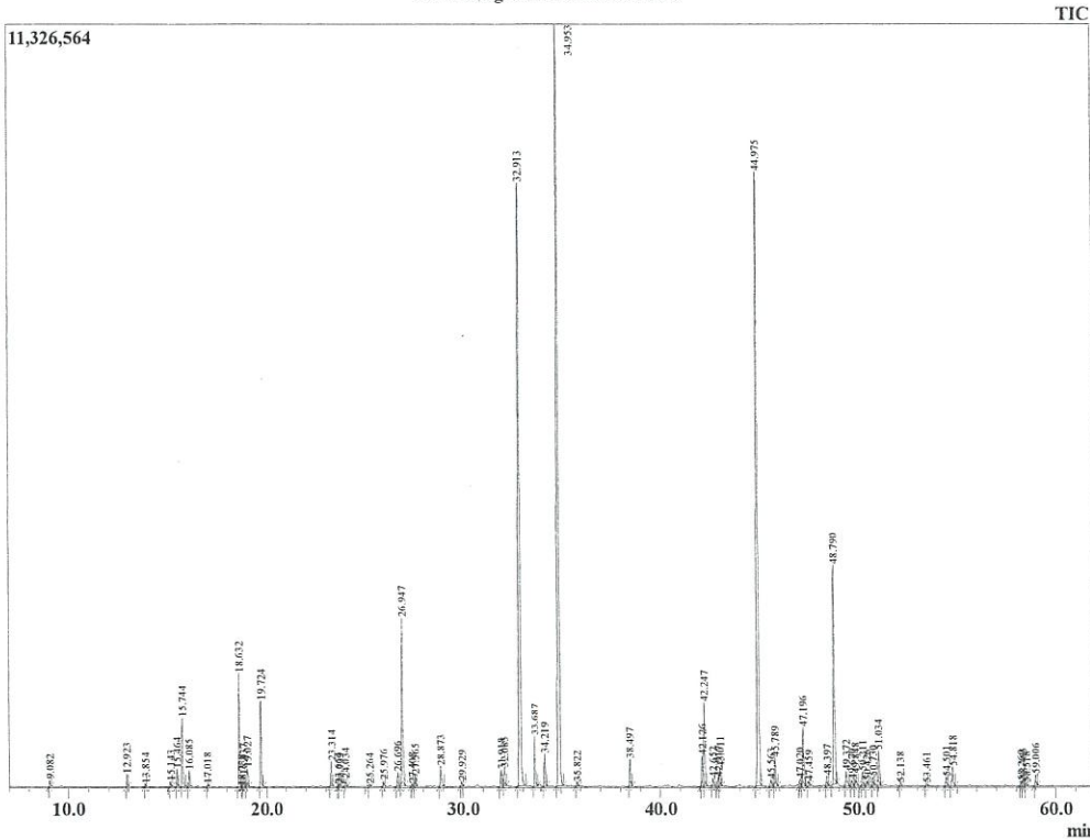
Chromatogram Melissa officinalis
