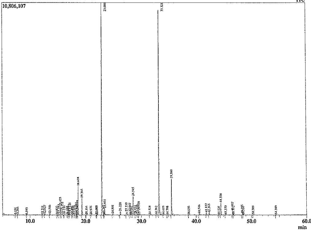
Chromatogram Lavandula angustifolia
